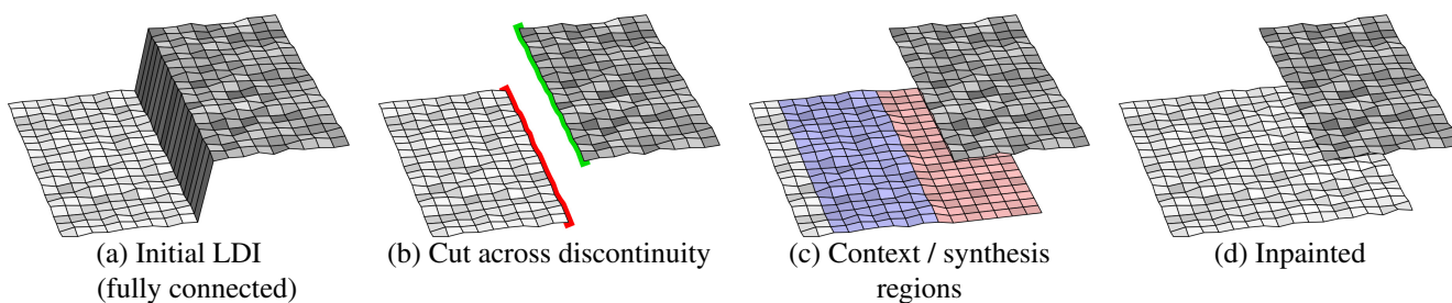
Figure 3. Conceptual illustration of the LDI inpainting algorithm. (a) The initial LDI is fully connected. A depth edge (discontinuity) is marked in gray. (b) We first cut the LDI pixel connections across the depth, forming a foreground silhouette (green) and a background silhouette (red). (c) For the background silhouette we spawn a context region (blue) and a synthesis region (red) of new LDI pixels. (d) The synthesized pixels have been merged into the LDI.
